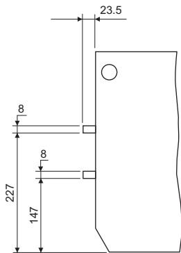
Terminal for 400/630/800 S1
