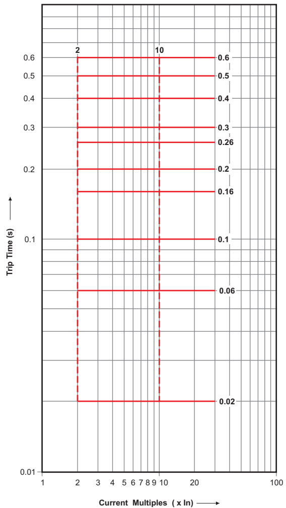
Short-Circuit (SR21i)
