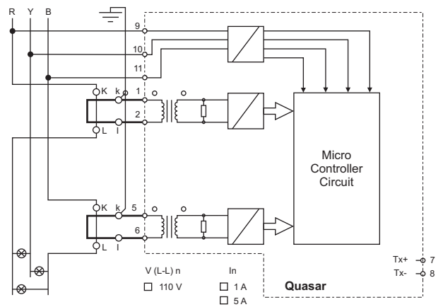
3 Ph.3 Wire with CT & without PT
