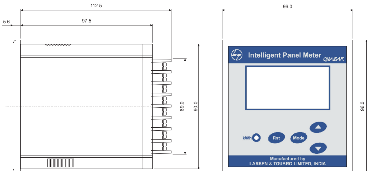
Panel Cutout 92 x 92 mm
