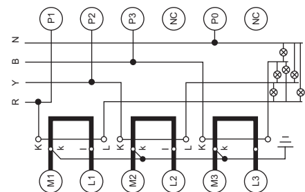
3 P 4 W with CT 240 V-1 A & 5 A
