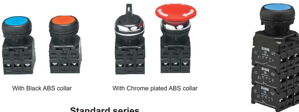
Gen Next actuator with snap fit contacts. Maximum 3 X 3 contacts
