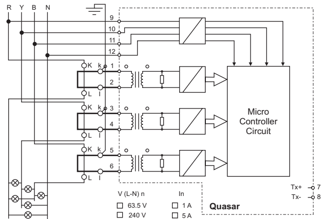
3 Ph. 4 Wire with CT & without PT
