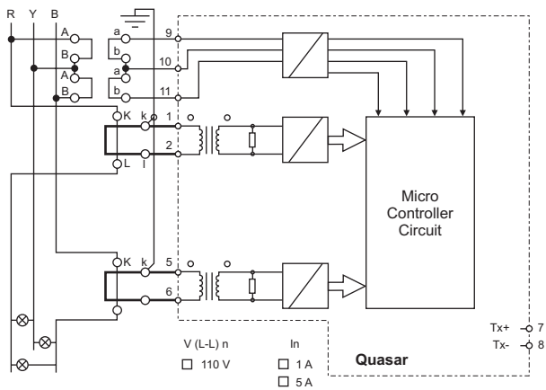
3 Ph. 3 Wire with CT & PT
