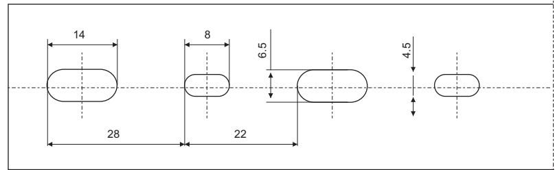
Bottom Mounting Slots for All Sizes
