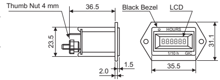
Screw Mount Bezel
