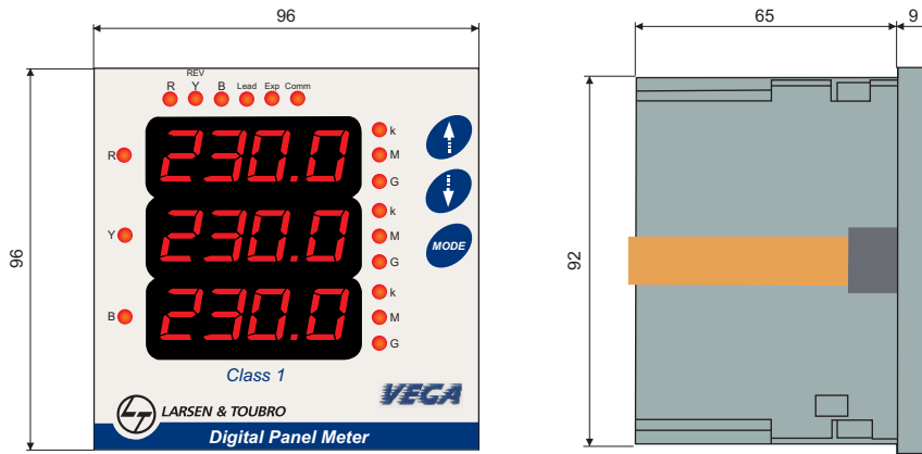
Panel Cutout Dimensions 92 mm x 92 mm
