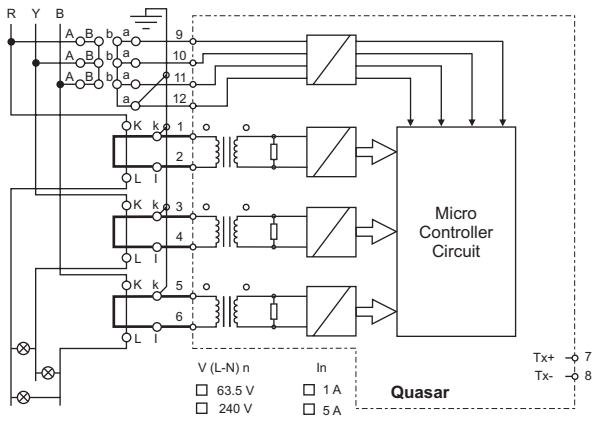
3 Ph. 4 Wire with CT & PT
