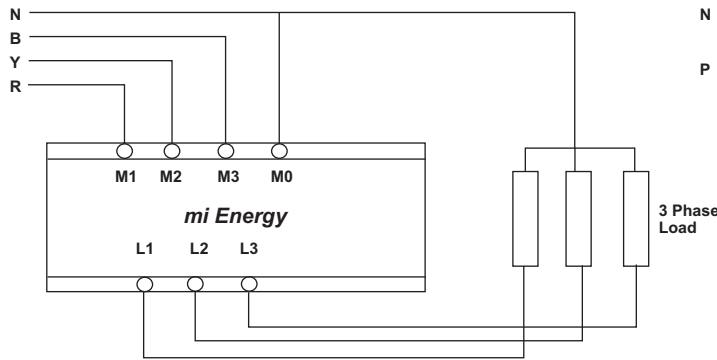
3-Phase
